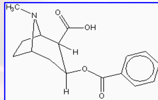
Benzoylecgonine
